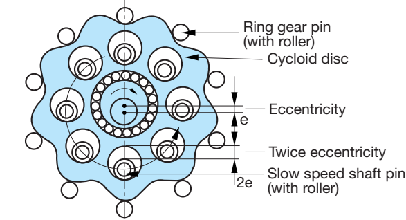
Fig. D-6 Combination of Planet-Sun Gears and Constant Speed Internal Gear
