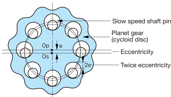
Fig. D-5 Constant Speed Internal Gearing
