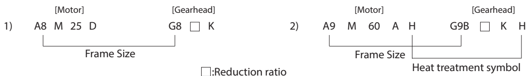
Fig.2 Combination ex. of motor and gearhead
